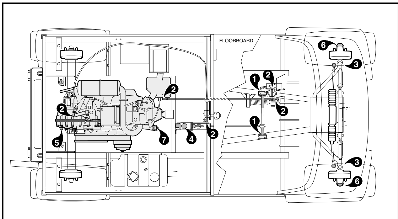
Figure 14 Lubrication Points
